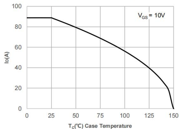
Figure 2: Current De-rating
