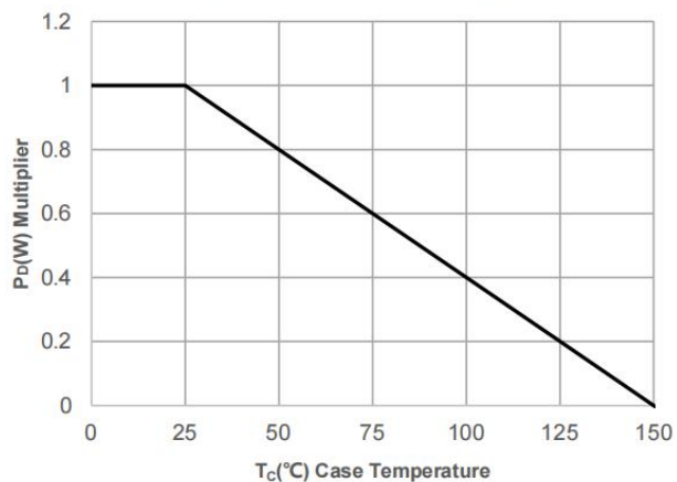
Figure 1: Power De-rating
