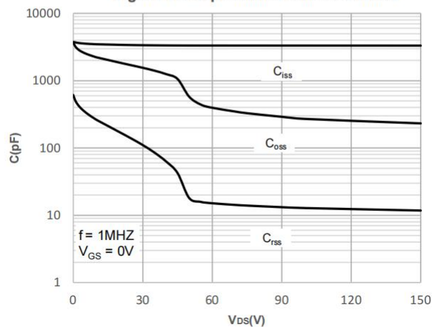
Figure 10: Capacitance Characteristics
