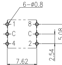
P.C.B DIMENSION (Top View)
