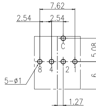
P.C.B DIMENSION (Top View)
