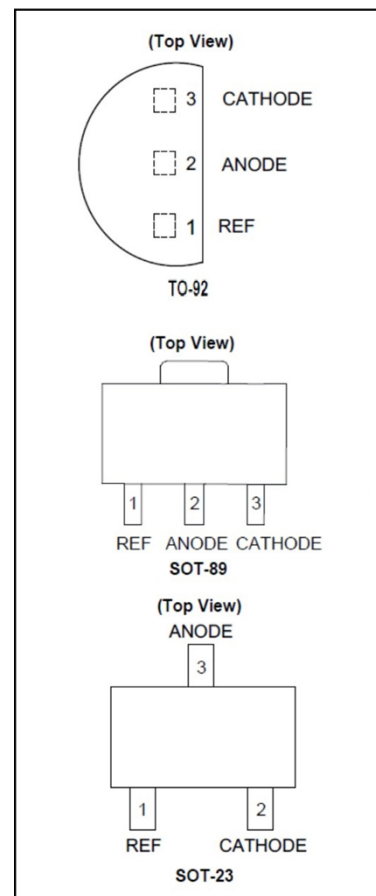
Pin Assignments
