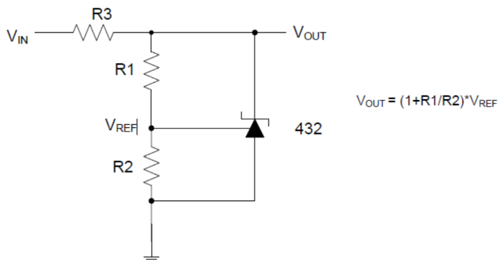
Shunt Regulator
