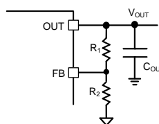
Fig. 5. V_{OUT} Programming
