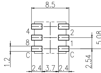
P.C.B DIMENSION (Top View)
