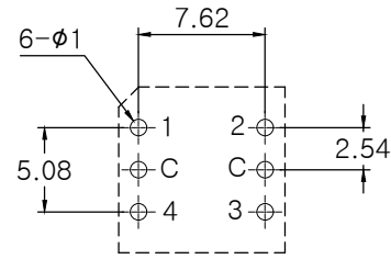
P.C.B DIMENSION (Top View)
