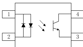
Pin Configuration
