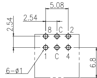
P.C.B DIMENSION (Top View)
