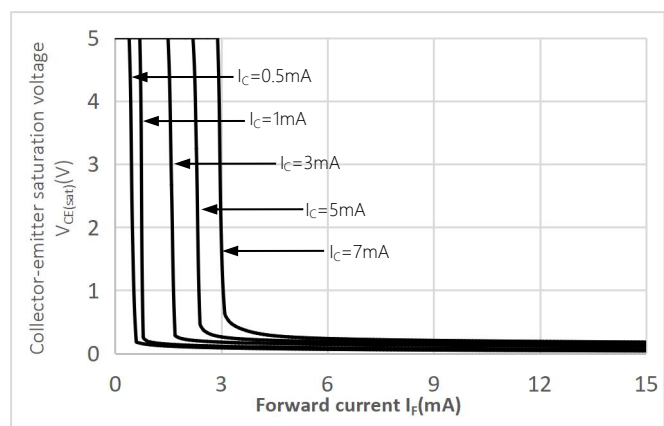
Fig.9 Collector-emitter Saturation Voltage vs Forward Current
