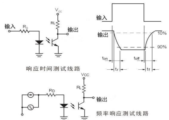
Fig.12 Switching Time Test Circuit & Waveforms
