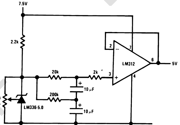
Low Noise Buffered Reference
