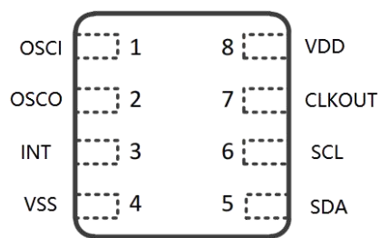
DFN-8 3*3
