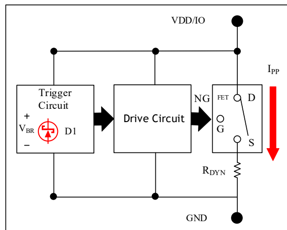
Fig. 2 The working principle of TDS
