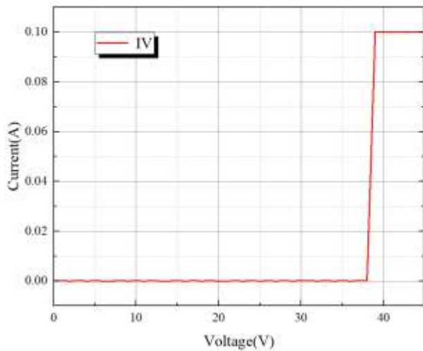
IV Characteristics
