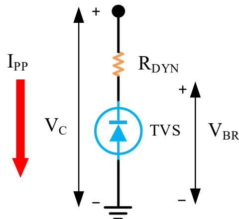
Fig.1 Equivalent circuit of traditional TVS diode
