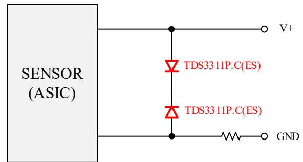
Fig. 6 Application of 2-wire sensor
