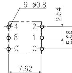
P.C.B DIMENSION (Top View)
