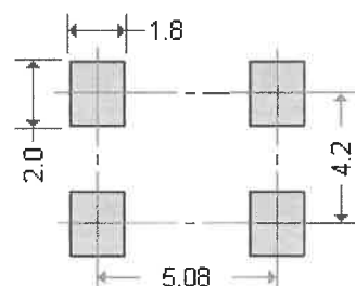
Land Pattern ( reference )
