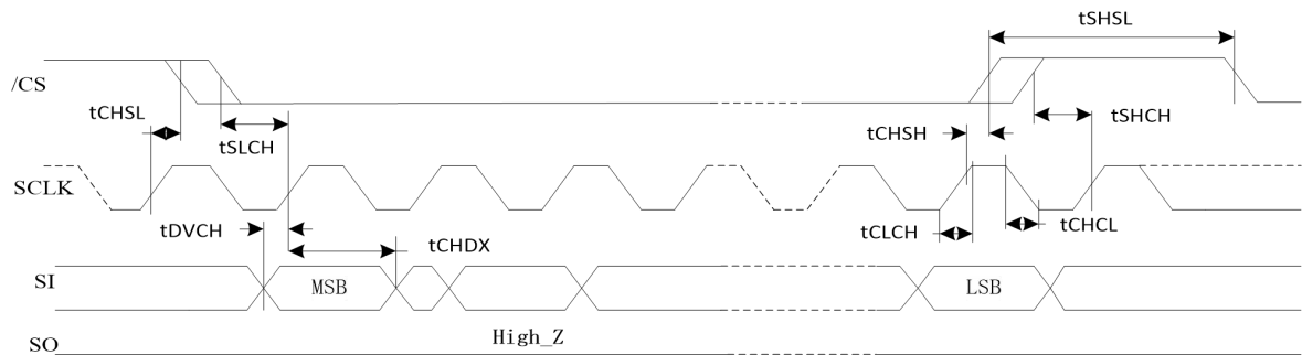
Figure 46. Serial inputTiming
