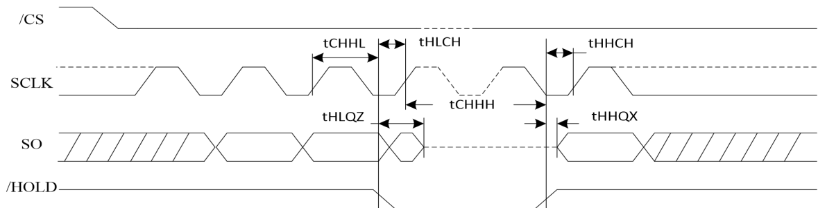
Figure 48. Hold Timing
