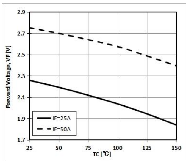
Figure 8: Typical Forward Voltage vs IF
