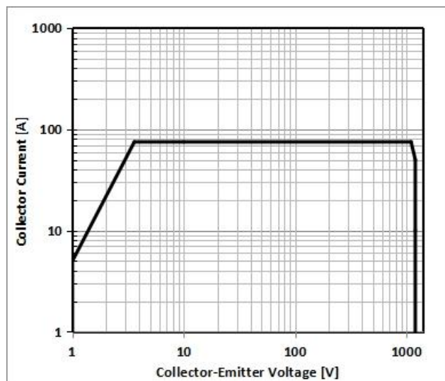
Figure 3: Reverse Bias SOA, T_J=150^{\circ}\text{C} , V_{GE}=15\text{V}
