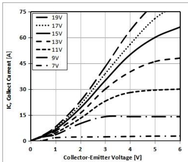
Figure 6: Typical IGBT Output characteristics, TC=150°C;tp=300us
