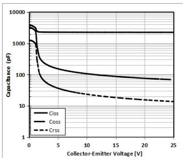
Figure 17: Typical Capacitance VS. VCE, VGE=0V,f=1MHz
