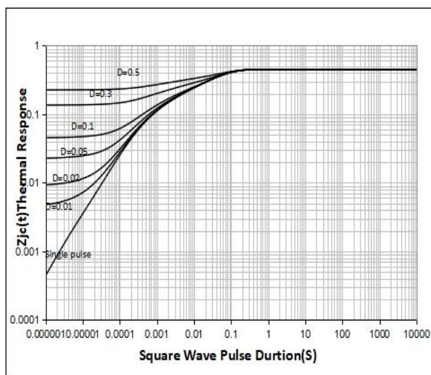
Figure 18: Normalized transient thermal impedance junction-to-case
