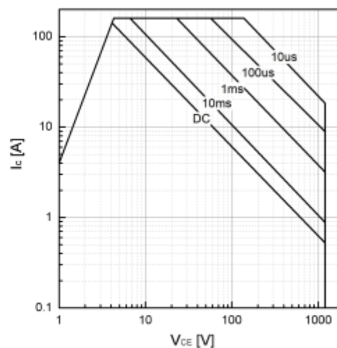
Fig 14. Safe operating area
