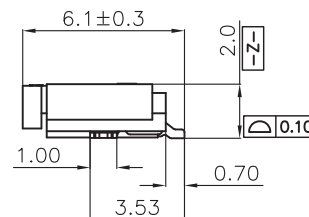
PART NO. LEGEND: F2GXXU-A1T5-AR
