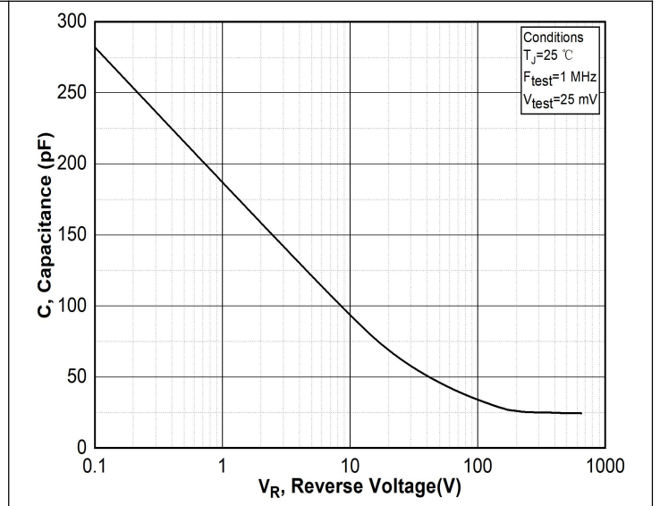
Figure 6. Capacitance Vs. Reverse Voltage
