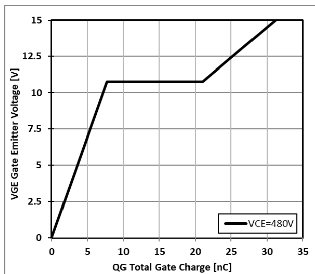
Figure 4: Typical Gate charge VS. V_{GE} , I_C=25\text{A}
