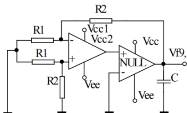
PSRR (+) = 20 \log \left| \frac{(Vcc1 - Vcc2)(1 + R2/R1)}{Vf9 - Vf10} \right|
