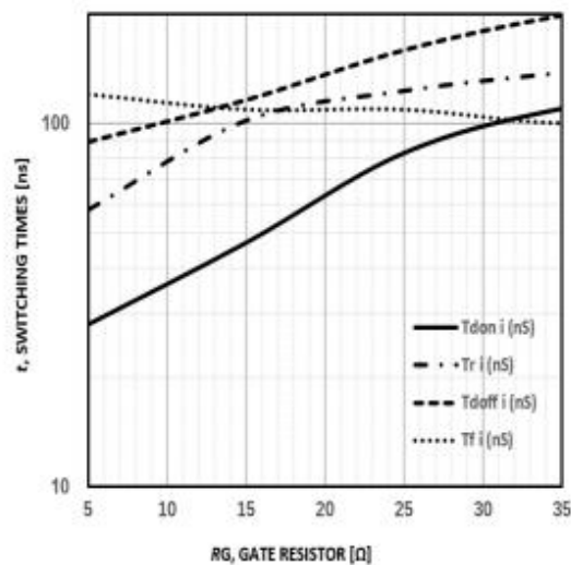
Figure10: Typical switching time VS. Rg, TC=25°C, VCE=600V, VGE=15V, IC=25A
