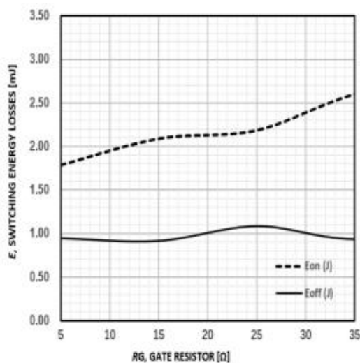
Figure9: Typical energy loss VS. Rg, TC=25°C, VCE=600V, VGE=15V, IC=25A
