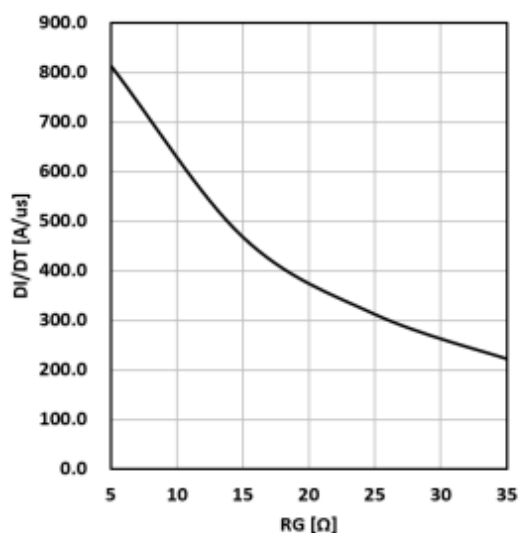
Figure 13. Typical diode di/dt vs rg Tc=25℃ VCE=600V VGE=15V IF=25A
