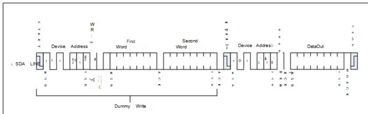
Figure 6-4 Random Read
