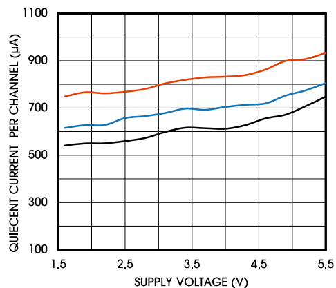
Figure 22. Per Channel Quiescent Current vs. Supply Voltage
