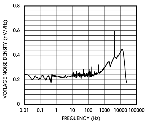
Figure 23. Voltage Noise Spectral Density vs. Frequency
