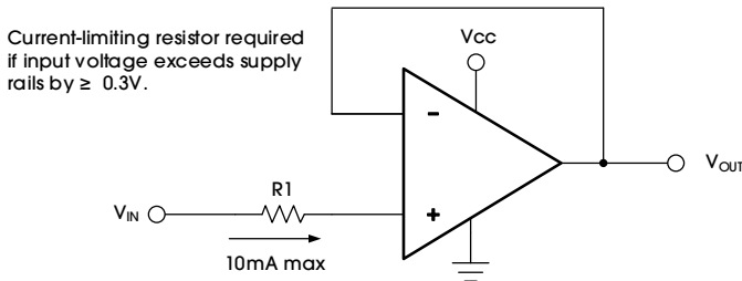
Figure 27. Input Current Protection
