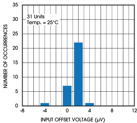
Figure 7. Offset Voltage Distribution, V_S = 5\text{V}
