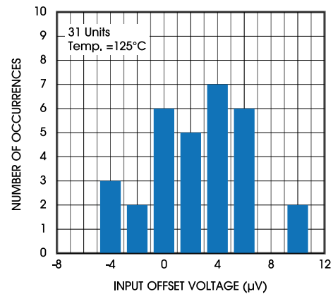
Figure 8. Offset Voltage Distribution, V_S = 5\text{V}
