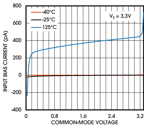
Figure 13. Input Bias Current on +IN Input Pin vs. Common-Mode Voltage
