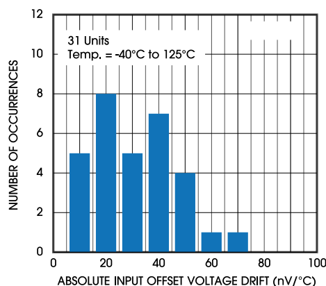
Figure 10. Offset Voltage Drift Distribution, V_s = 5V
