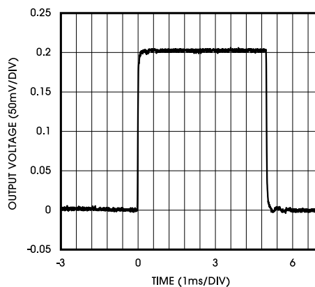
Figure 25. Small Signal Response, 3.3V
