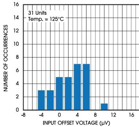
Figure 5. Offset Voltage Distribution, V_S = 3.3\text{V}
