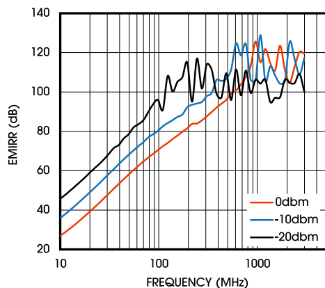
Figure 21. EMIRR Performance
