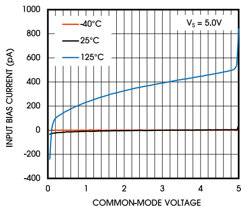
Figure 14. Input Bias Current on +IN Input Pin vs. Common-Mode Voltage
