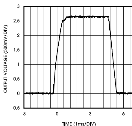
Figure 24. Large-Signal Response, 3.3V
