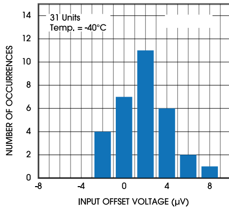
Figure 3. Offset Voltage Distribution, V_S = 3.3\text{V}
