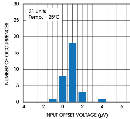
Figure 4. Offset Voltage Distribution, V_S = 3.3\text{V}
