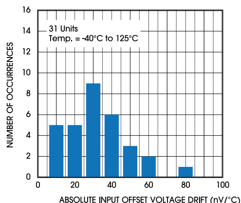
Figure 9. Offset Voltage Drift Distribution, V_s = 3.3V
