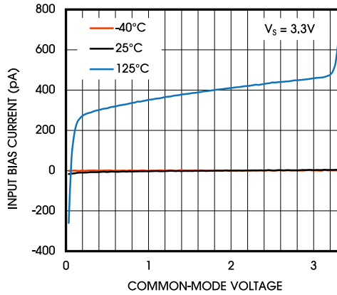
Figure 15. Input Bias Current on -IN Pin vs. Common Mode Voltage
