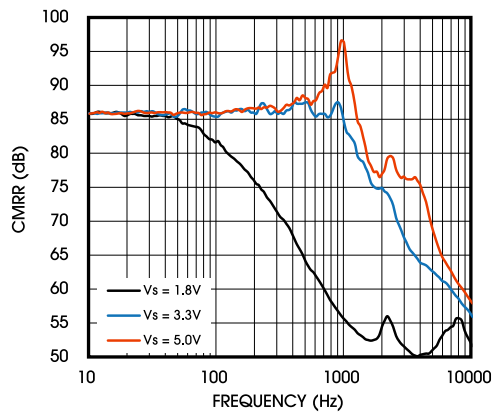
Figure 19. CMRR vs. Frequency
