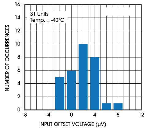
Figure 6. Offset Voltage Distribution, V_S = 5\text{V}
