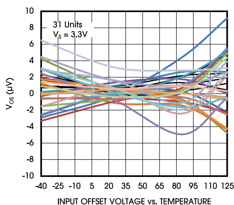
Figure 11. Offset Voltage vs Temperature, V_s = 3.3V
