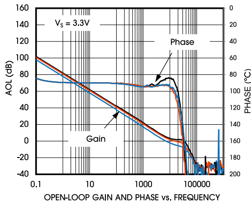
Figure 17. Open-Loop Gain and Phase vs. Frequency
