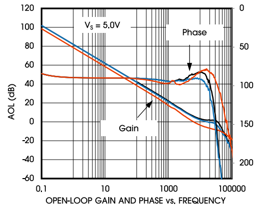
Figure 18. Open-Loop Gain and Phase vs. Frequency
