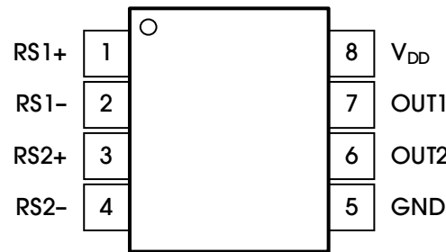
Figure 1. Pin Configuration
