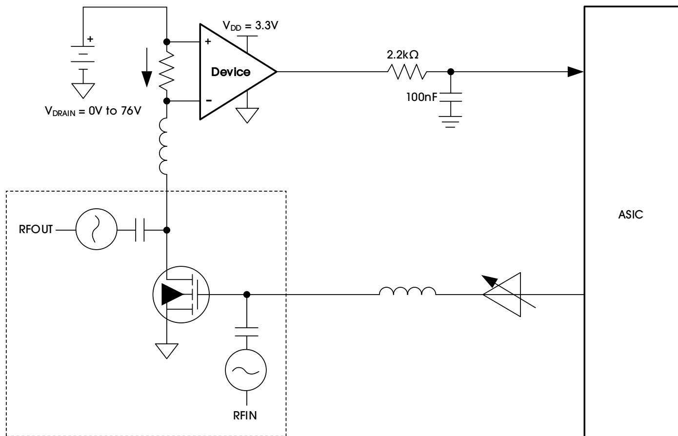
Figure 13. CSA2202 Used in Base-Station Application
