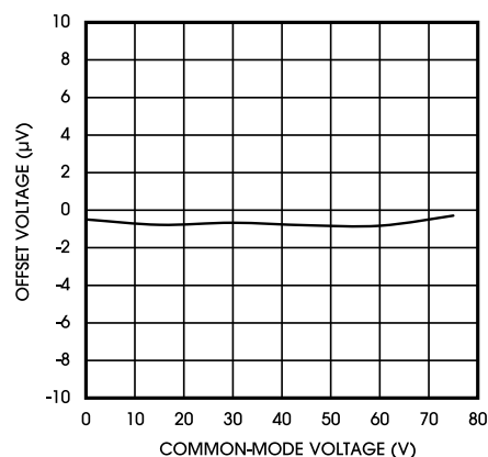
Figure 5. Input Offset Voltage vs. Input Common Mode Voltage
