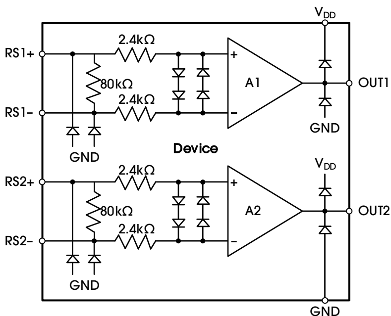
Figure 12. Functional Block Diagram
