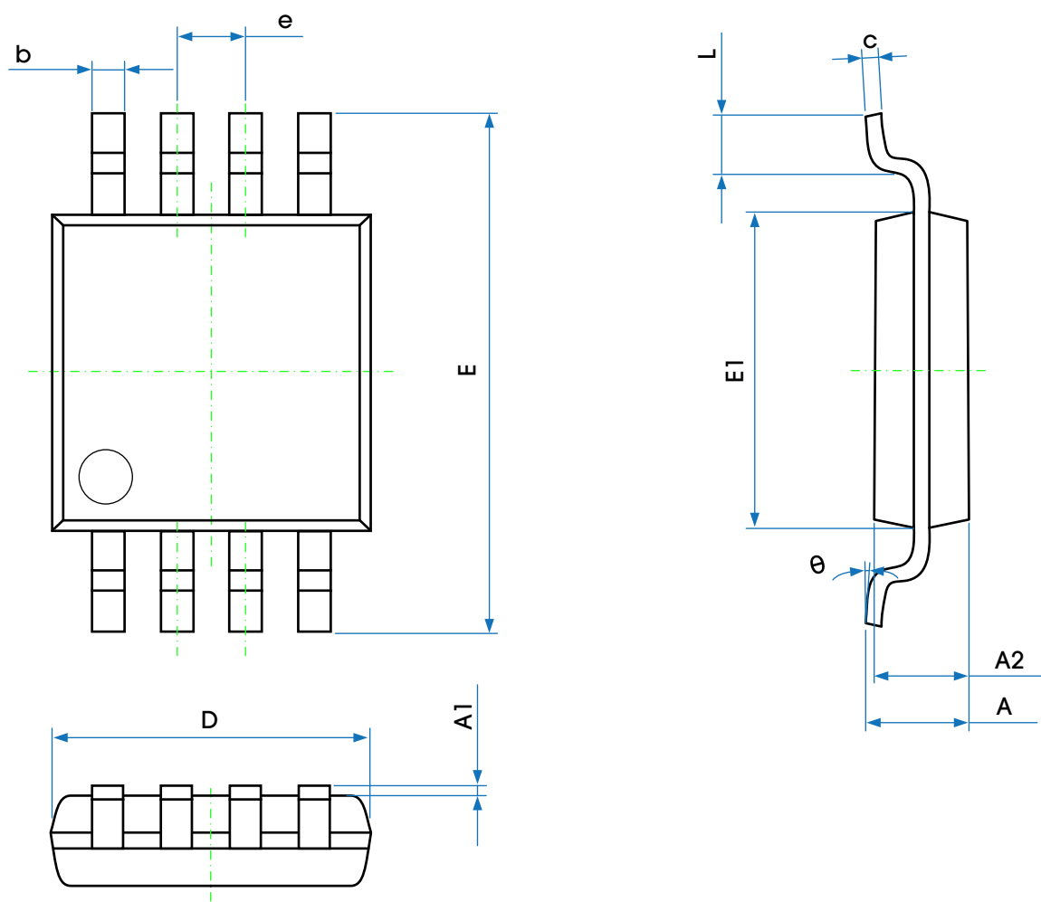
Figure 14. Package View
