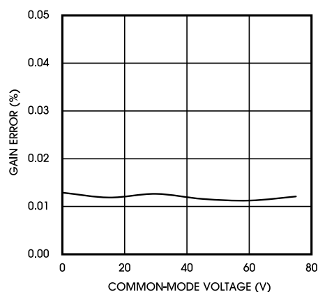
Figure 7. Gain Error vs. Common Mode Voltage
