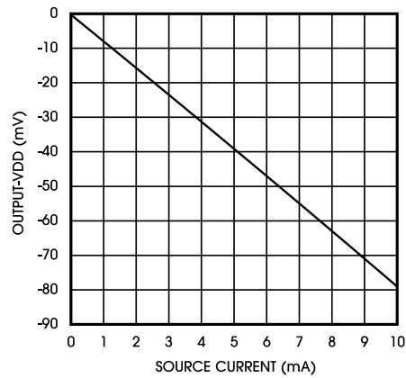
Figure 8. V_{OH} vs. Source Current
