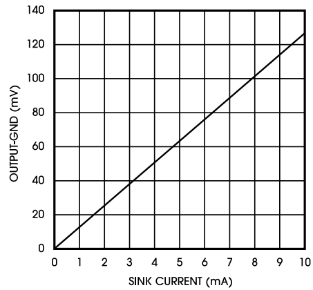
Figure 9. V_{OL} vs. Sink Current
