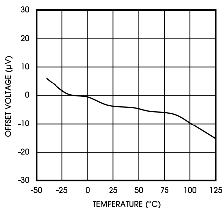
Figure 4. Input Offset Voltage vs. Temperature
