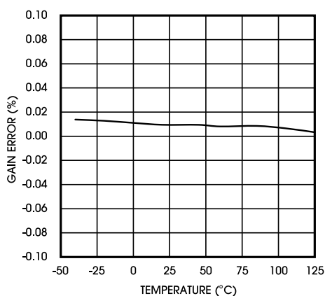
Figure 6. Gian Error vs. Temperature
