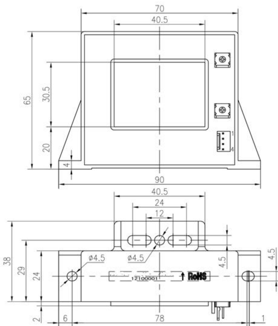
NCA1J-800A/SP1 电压传感器外形图 Dimensions NCA1J-800A/SP1 Series (in mm)
