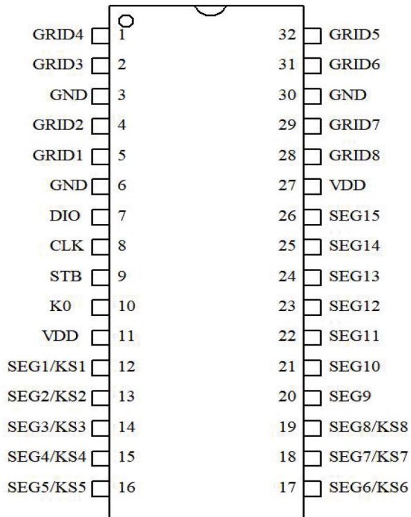
HTM1629C-TD 32SOP
