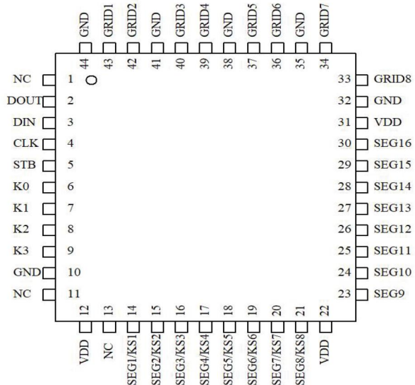
HTM1629E-TD 44LQFP
