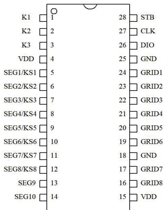
HTM1638-TD 28SOP/28SSOP
