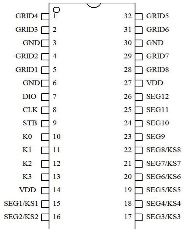
HTM1629D-TD 32SOP
