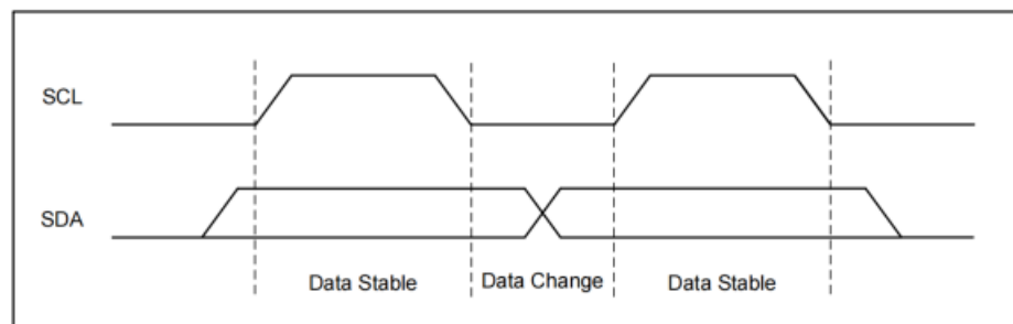
Figure 4-1 Data Validity
