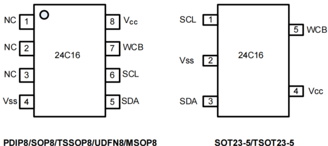
Figure 1-1 Pin Configuration
