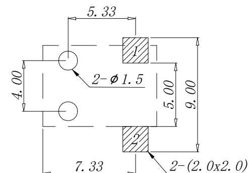
PCB. WELDING DRAWING (TOLERANCE: \pm 0.05 )
