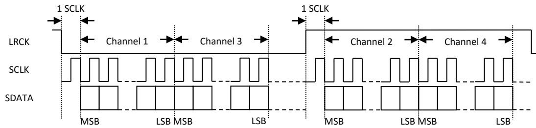
Figure 2e TDM I²S Serial Audio Data Format
