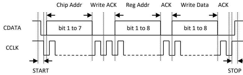
Figure 1a I²C Write Timing
