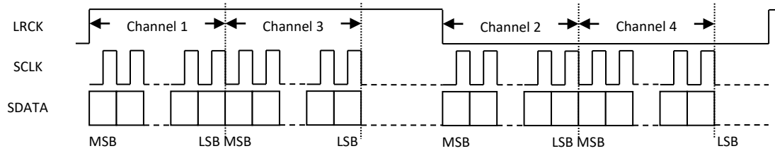
Figure 2e TDM I²S Serial Audio Data Format
