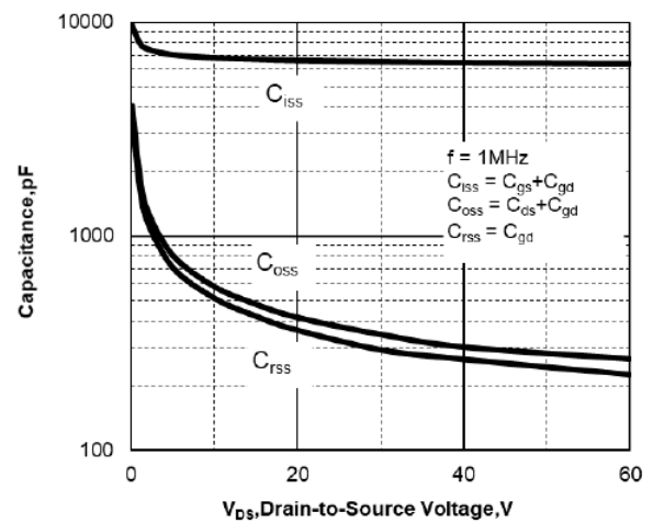
Fig 6: Capacitance Characteristics
