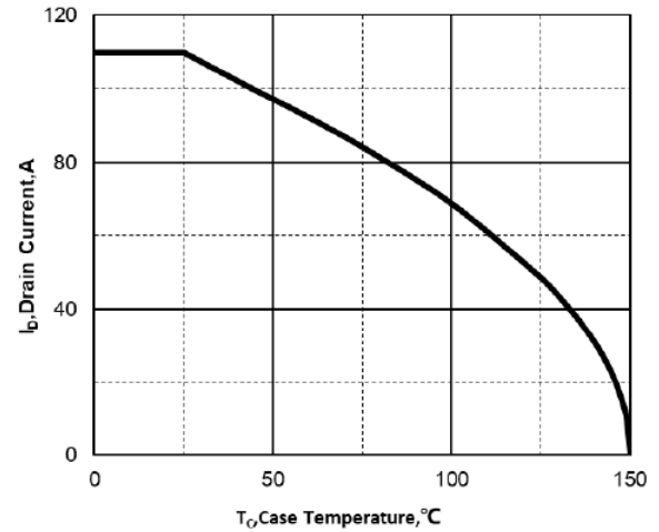
Fig 4: Maximum Continuous Drain Current VS. Case Temperature
