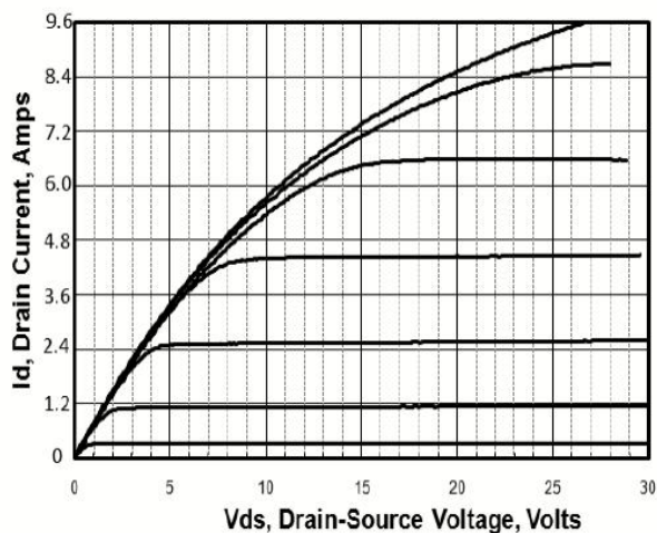
Figure 4. Output Characteristics
