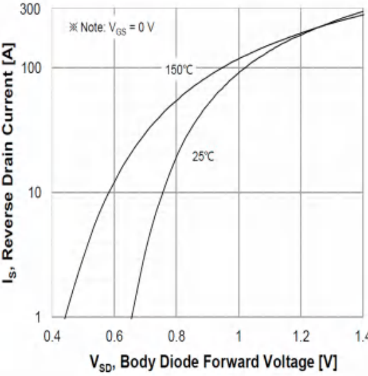
Forward characteristics of reverse diode
