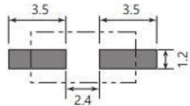
Land Pattern
