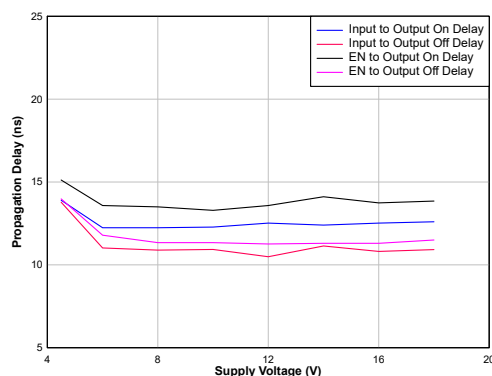
Figure 16. Propagation Delay vs. Supply Voltage
