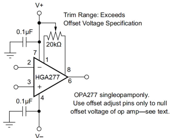
Figure 24. HG277 Offset Voltage Trim Circuit
