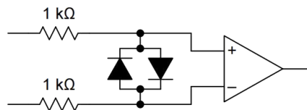
Figure 25. HGx277 Input Protection
