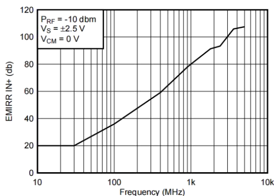
Figure 27. HG277 EMIRR IN+ vs Frequency
