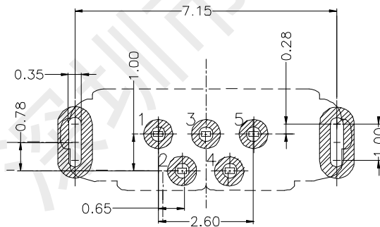
RECOMMENDED PCB LAYOUT(TOP VIEW) GENERAL TOLERANCES:±0.05
