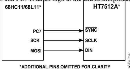
Figure 29. HT7512A to 68HC11/68L11 Interface
