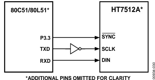
Figure 30. HT7512A to 80C51/80L51 Interface
