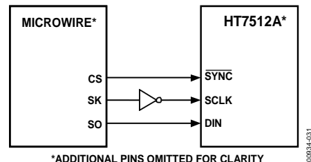
Figure 31. HT7512A to MICROWIRE Interface
