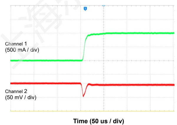
Channel 1 = I_{OUT} , channel 2 = V_{OUT} , V_{IN} = 1.8V , V_{OUT} = 0.8V Figure 17. Load Transient (1 mA to 1000 mA)
