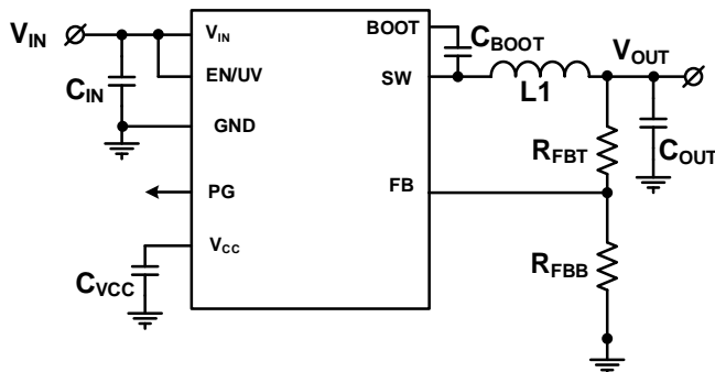
Fig.1 Schematic Diagram
