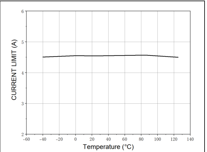
Fig.5 Current Limit VS. Junction Temperature at Duty = 40%
