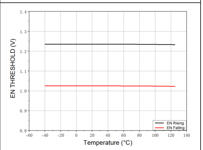
Fig.9 EN Threshold VS. Junction Temperature
