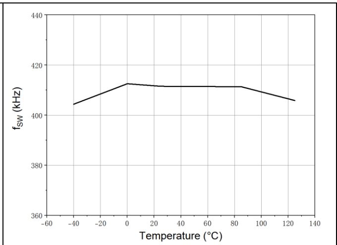
Fig.11 Switching Frequency VS. Junction Temperature
