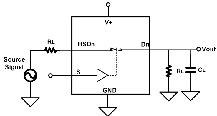
-3dB Bandwidth
