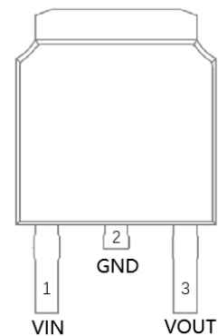
TO-252
