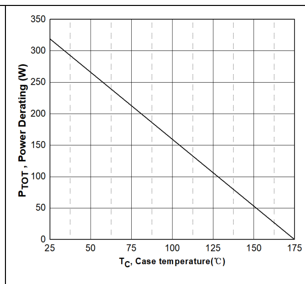
Figure 4. Power Derating
