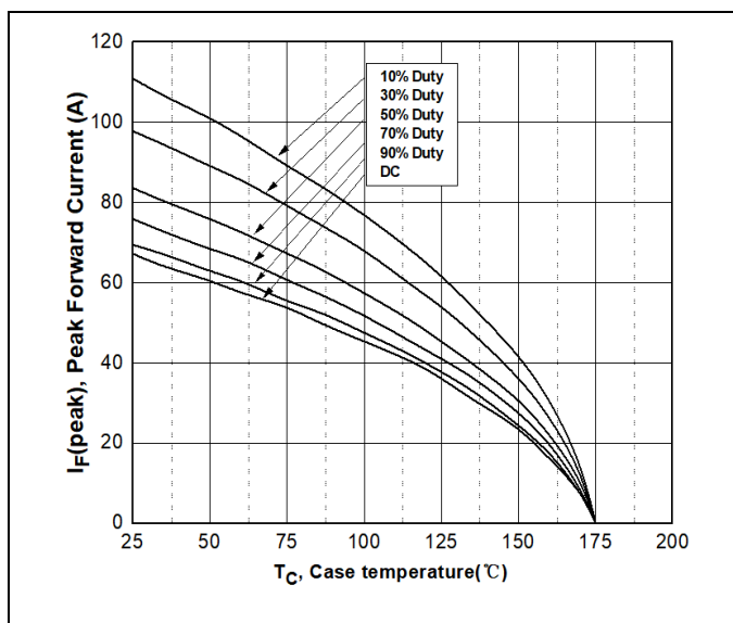
Figure 3. Current Derating
