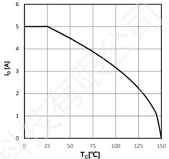
Figure 10: Drain current
