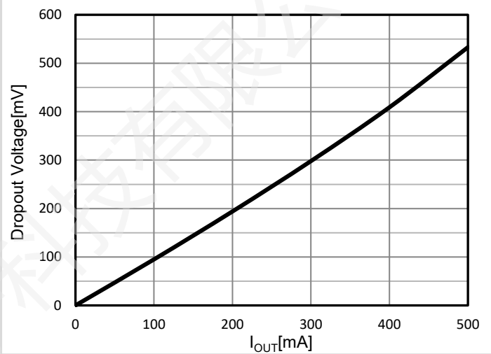
6. Dropout Voltage ( V_{OUT} = 95\% \times 2.8V , I_{OUT} = 0 \rightarrow 500mA )
