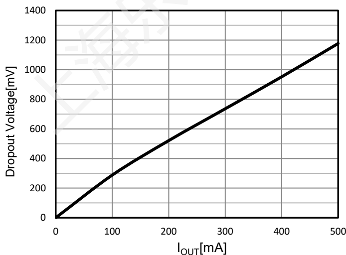
7. Dropout Voltage ( V_{OUT} = 95\% \times 1.2V , I_{OUT} = 0 \rightarrow 500mA )
