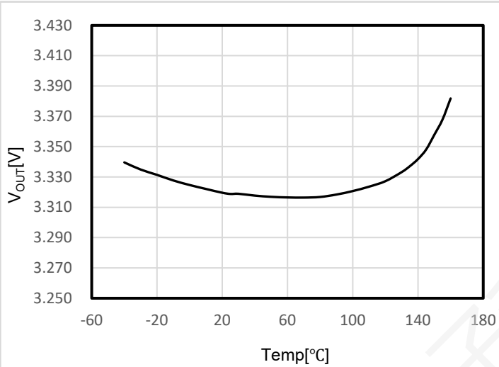
1. V_{OUT} vs Temperature ( V_{IN}=4.3\text{V} , V_{OUT}=3.3\text{V} , I_{OUT}=1\text{mA} )
