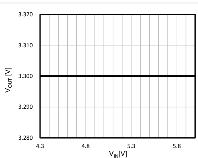
4. V_{OUT} vs V_{IN} ( V_{IN}=4.3\text{V} \rightarrow 6.0\text{V} , V_{OUT}=3.3\text{V} , I_{OUT}=1\text{mA} )
