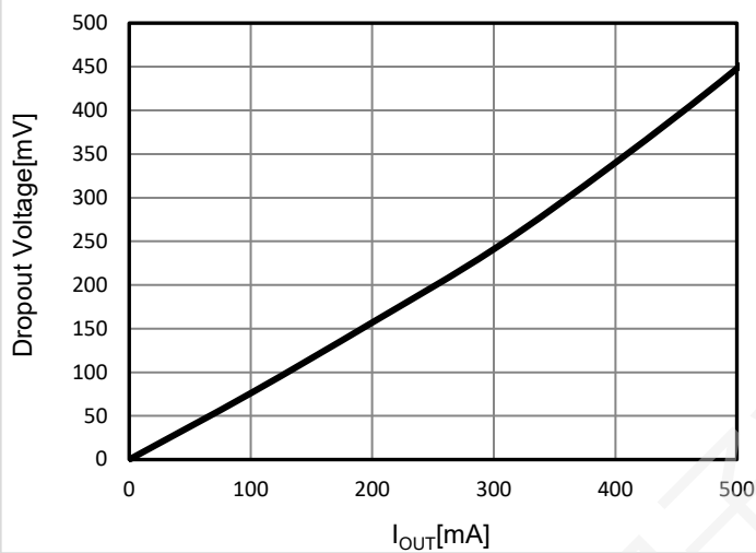
5. Dropout Voltage ( V_{OUT} = 95\% \times 3.3V , I_{OUT} = 0 \rightarrow 500mA )
