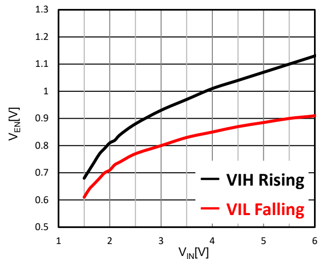
8. V_{EN} Thresholds vs V_{IN} ( V_{OUT} = 3.3V , I_{OUT} = 0mA )
