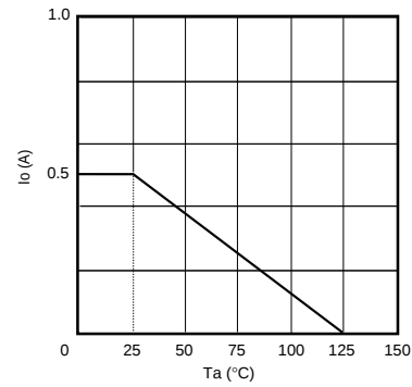
Fig.4 Derating curve
