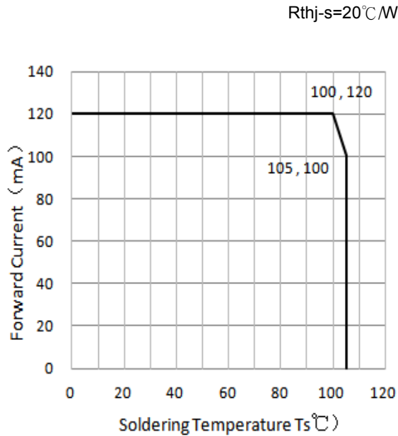
Soldering Temperature VS Allowable Forward Current 焊盘温度与允许电流特性
