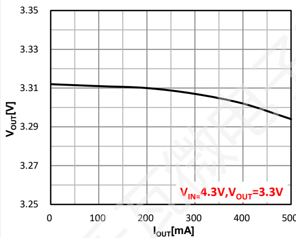
Figure 15. Load Regulation
