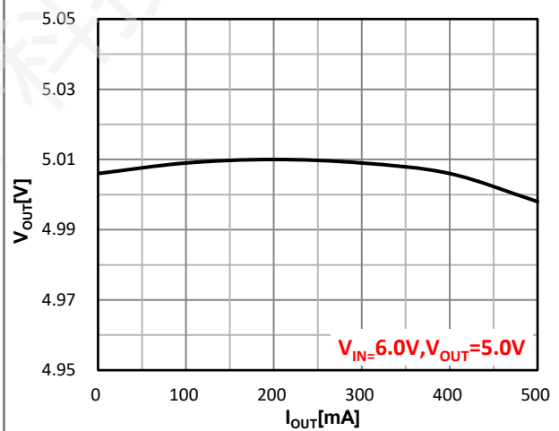
Figure 16. Load Regulation
